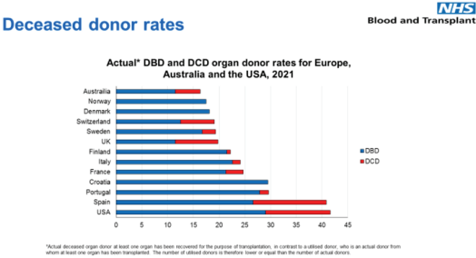
Figure 1. Relative contributions of donation after brain death (DBD) and donation after circulatory death (DCD) to deceased donation in various countries around the world, as measured by donors per million population (pmp) in 2021. Source: Council of Europe – Transplant Newsletter
