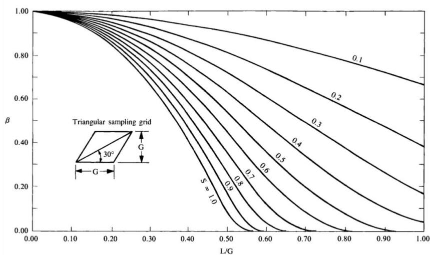
Figure 10.5 Curves relating L/G to consumer's risk, \beta , for different target shapes when sampling is on a triangular grid pattern (after Zirschky and Gilbert, 1984, Fig. 4).
